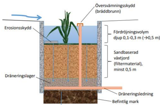
Figur 28 Principskiss regnbädd (Water Revival Systems)
