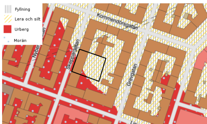
Jordartskarta, SGU
